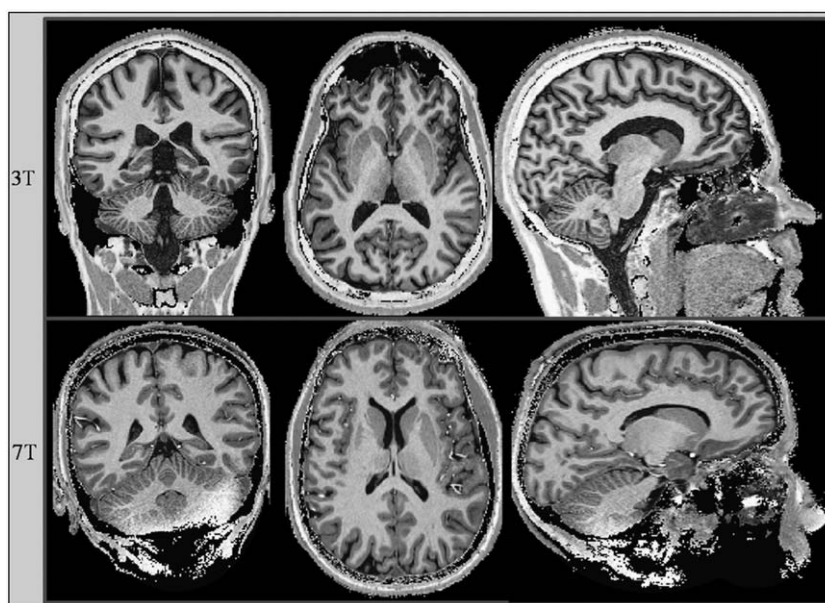
Fig. 5. Transverse, coronal, and sagittal slices taken from images acquired at 3 T (top) and 7 T (bottom). Three-Tesla data were acquired with MP2RAGE _{TR}/T_1/T_2 = 6.25 s/0.8 s/2.2 s, \alpha_1/\alpha_2 = 4^\circ/5^\circ , 1 mm 3 without fat suppression. Seven-Tesla data were acquired with MP2RAGE _{TR}/T_1/T_2 = 8.0 s/1.0 s/4.0 s, \alpha_1/\alpha_2 = 4^\circ/5^\circ , 0.73 mm 3 with fat suppression. Background was suppressed using a mask based on the thresholding of the second contrast image.
