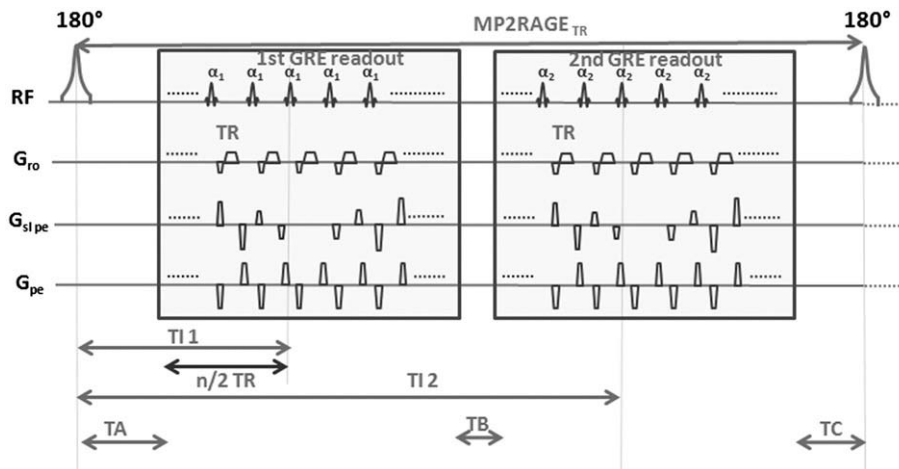
Fig. 1. Diagram of the MP2RAGE sequence. Inversion times T_1 and T_2 are defined as the time from the middle of the inversion pulse to the excitation corresponding to the center k-space line in the phase encoding in the slab selection direction. MP2RAGE TR is the time between two successive inversion pulses and TR is the time between successive excitation pulses in the GRE kernel, which is composed of n excitations.
