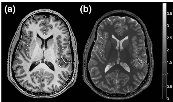
Fig. 9. Isotropic 0.65-mm resolution MP2RAGE (a) and T_1 (b) transverse slice taken from a 3D dataset obtained at 7 T with the following parameters: MP2RAGE-TR/ TI_1 / TI_2 = 8.0/1.0/3.2 s \alpha_1/\alpha_2 = 4^\circ/4^\circ . The number of excitations per GRE block was 256, the BW was 200Hz/px, and total acquisition time was 12 min.
