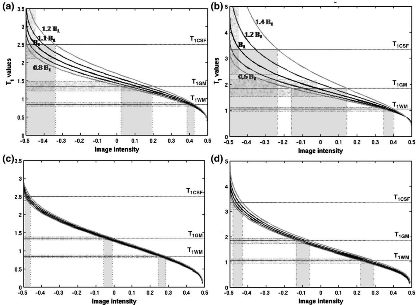
Fig. 3. The effect of B_1^+ deviations on signal intensities and T_1 estimations. The plots show signal intensity versus T_1 values considering different MP2RAGE parameters: (a) MP2RAGE_{TR} = 6.25 s, TI_1/TI_2 = 0.8/3.2 s, \alpha_1/\alpha_2 = 7^\circ/5^\circ ; (c) MP2RAGE_{TR} = 6.25 s, TI_1/TI_2 = 0.8/3.2 s, \alpha_1/\alpha_2 = 4^\circ/5^\circ ; (b) MP2RAGE_{TR} = 8.0 s, TI_1/TI_2 = 1.0/3.3 s, \alpha_1/\alpha_2 = 7^\circ/5^\circ ; (d) MP2RAGE_{TR} = 8.0 s, TI_1/TI_2 = 1.0/3.3 s, \alpha_1/\alpha_2 = 4^\circ/5^\circ . Plots a, c and b, d correspond to 3T and 7T parameters, respectively. The assumed CSF, GM, and WM T_1 values at those fields are shown as horizontal lines. Dark grey and light grey lines in the plots show the expected signal as a function of T_1 for an effective transmission field deviation of (a, c) \pm 10\% , \pm 20\% and (b, d) \pm 20\% , \pm 40\% . Light grey boxes show the predicted spread of signal intensities (vertical boxes) and T_1 estimations (horizontal boxes) of the different tissues due to B_1 variations of (a, c) \pm 20\% and (b, d) \pm 40\% .
